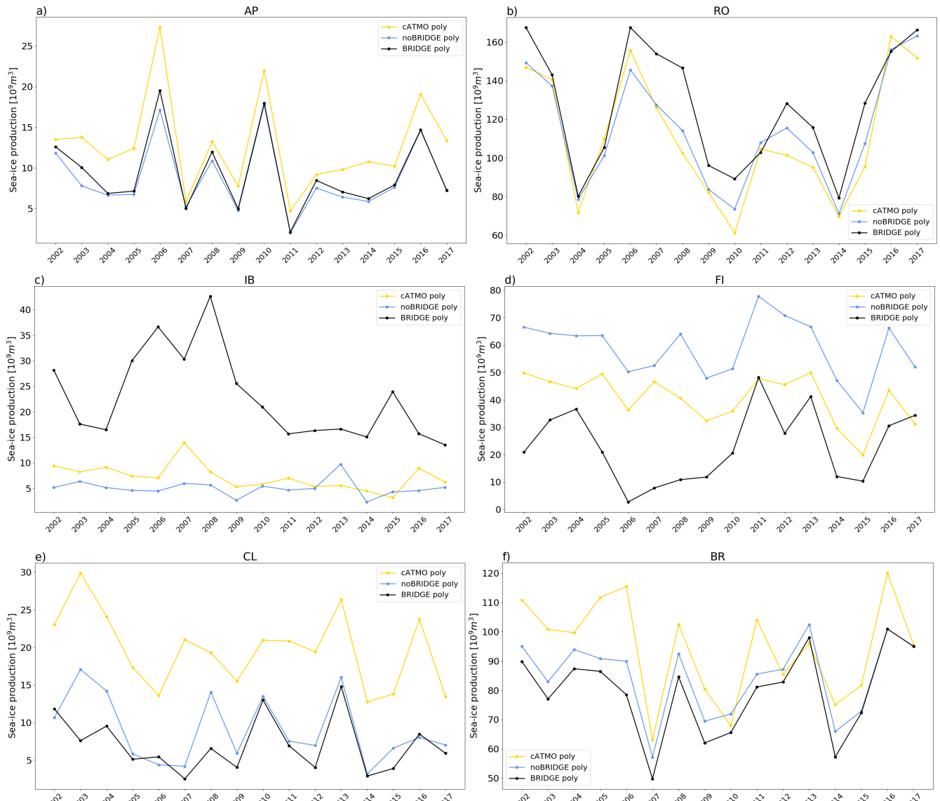
Supplement figure 1. Time-series of the cumulative polynya ice-production (2002–2017) in the southern Weddell Sea from FESOM experiments for the six sub-regions shown in Fig.1.
