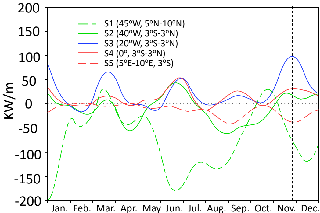
(a) Energy flux : BCM1
