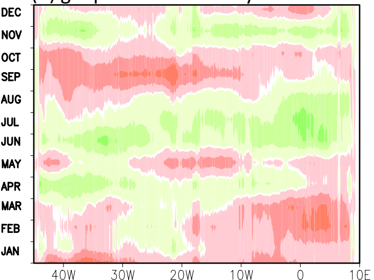
(h) geopotential anomaly : BCM4
