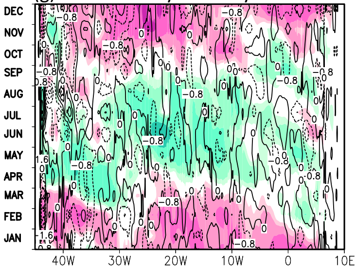
(g) zonal velocity anomaly : BCM4
