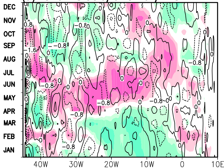
(c) zonal velocity anomaly : BCM2
