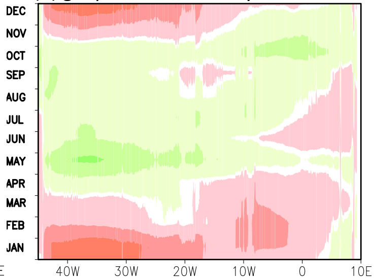
(h) geopotential anomaly : BCM4
