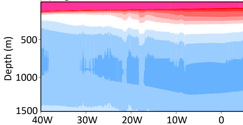
(b) Eigenfunction: BCM2
