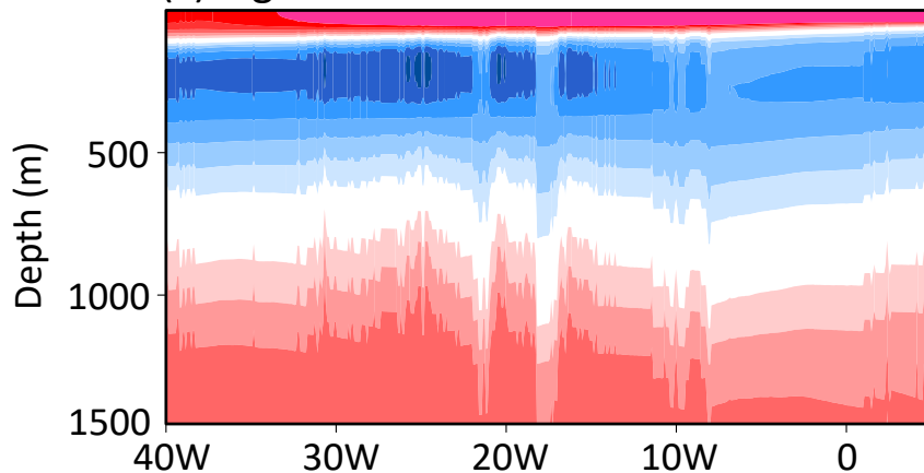
(c) Eigenfunction: BCM3
