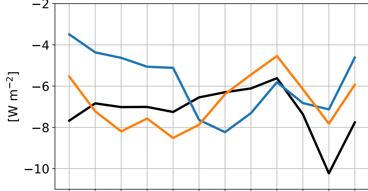
Sensible heat flux
