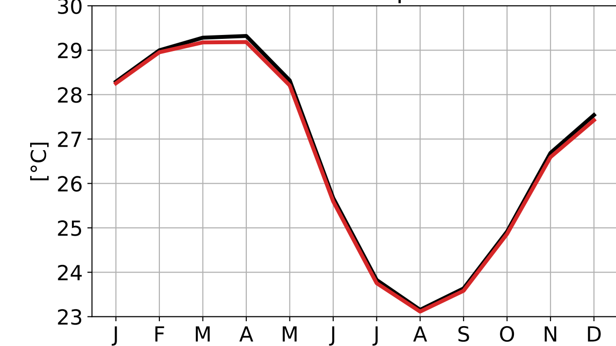
Sea surface temperatures
