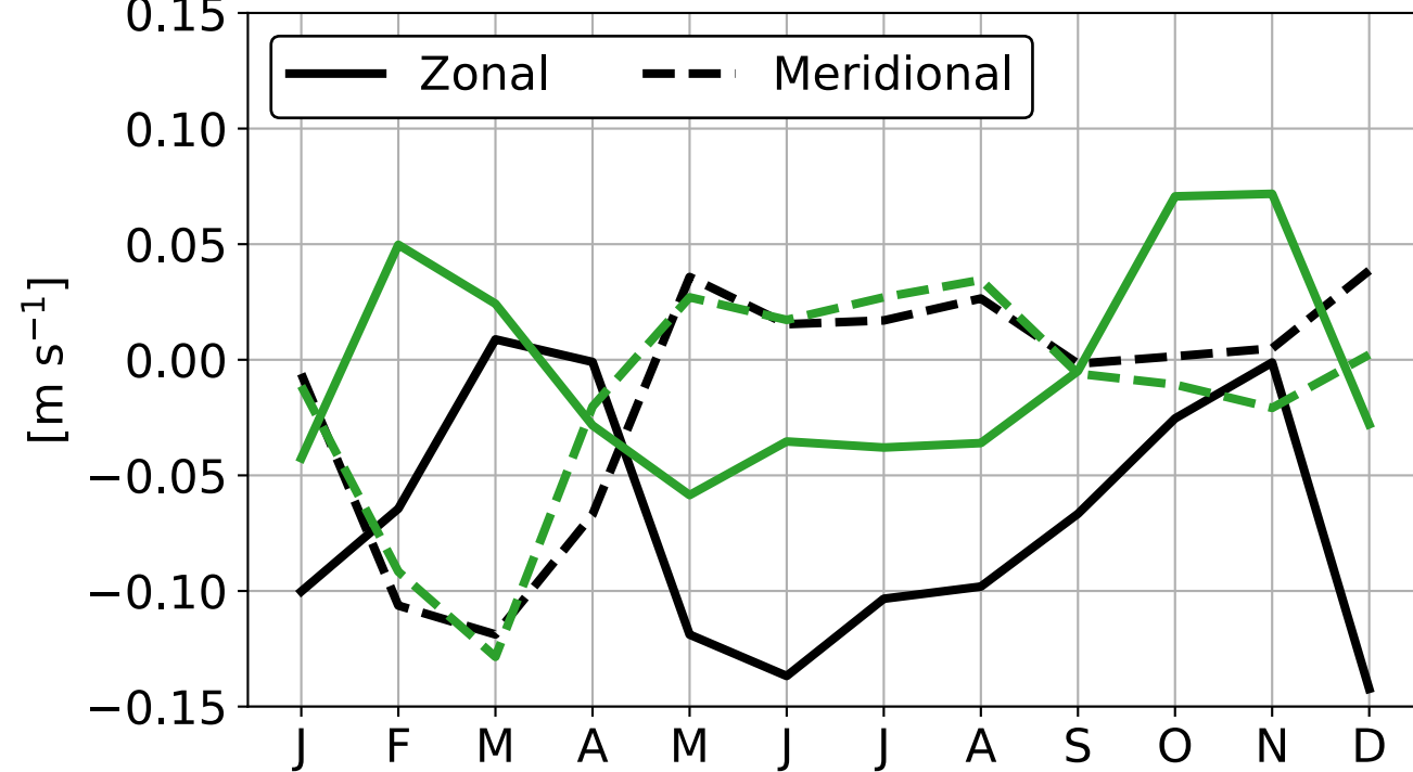
Horizontal Velocities
