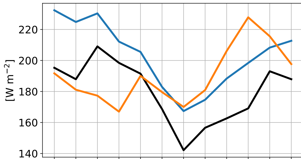
Shortwave radiation
