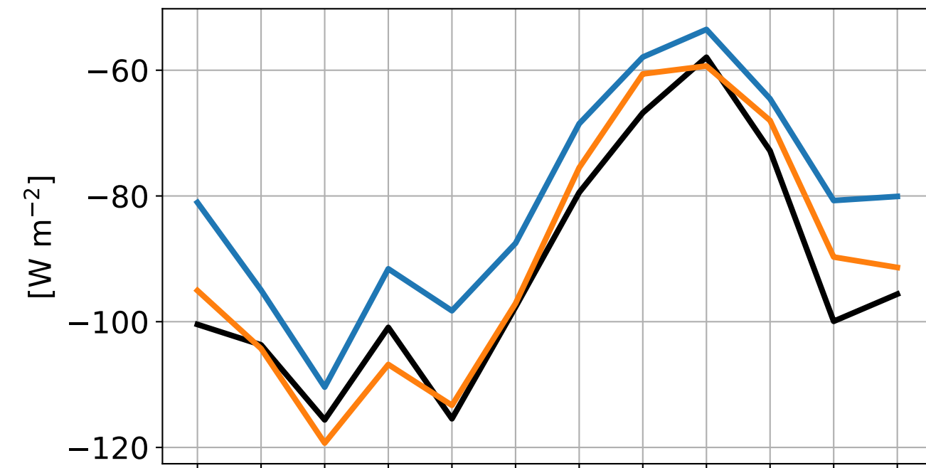
Latent heat flux
