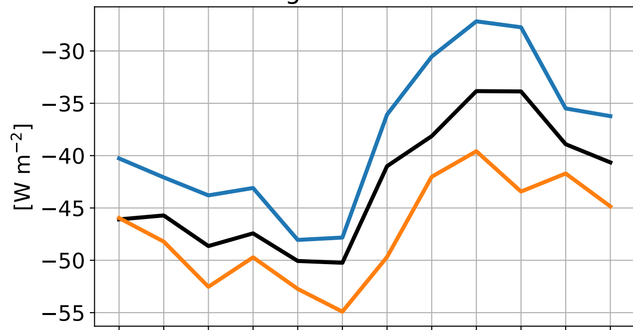
Longwave radiation
