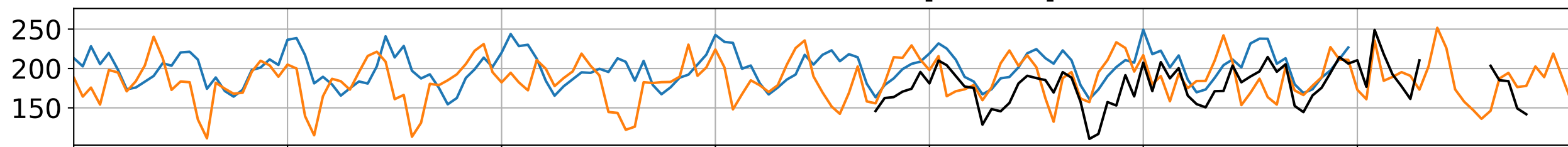
Longwave radiation [ \text{W m}^{-2} ]
