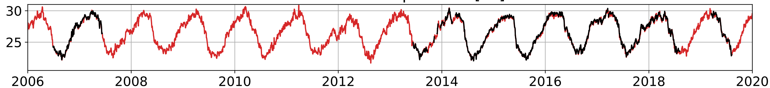
Sea surface temperature [ ^{\circ}\text{C} ]
