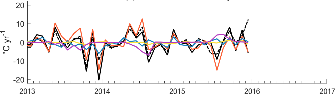
(b) Southern cold anomaly
