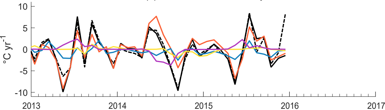
(a) Northern cold anomaly
