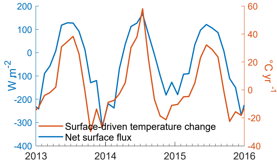
(b) Surface heat flux: south
