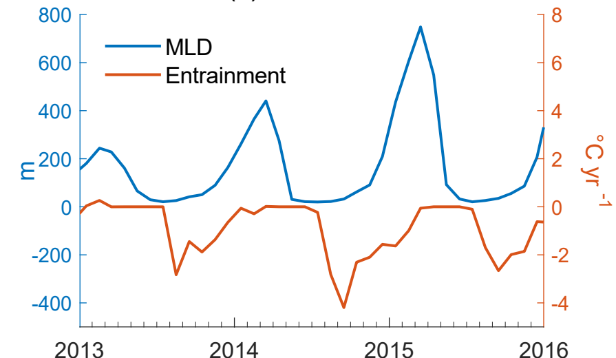
(c) MLD: north
