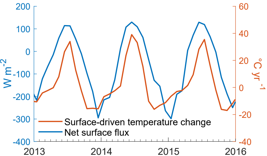
(a) Surface heat flux: north
