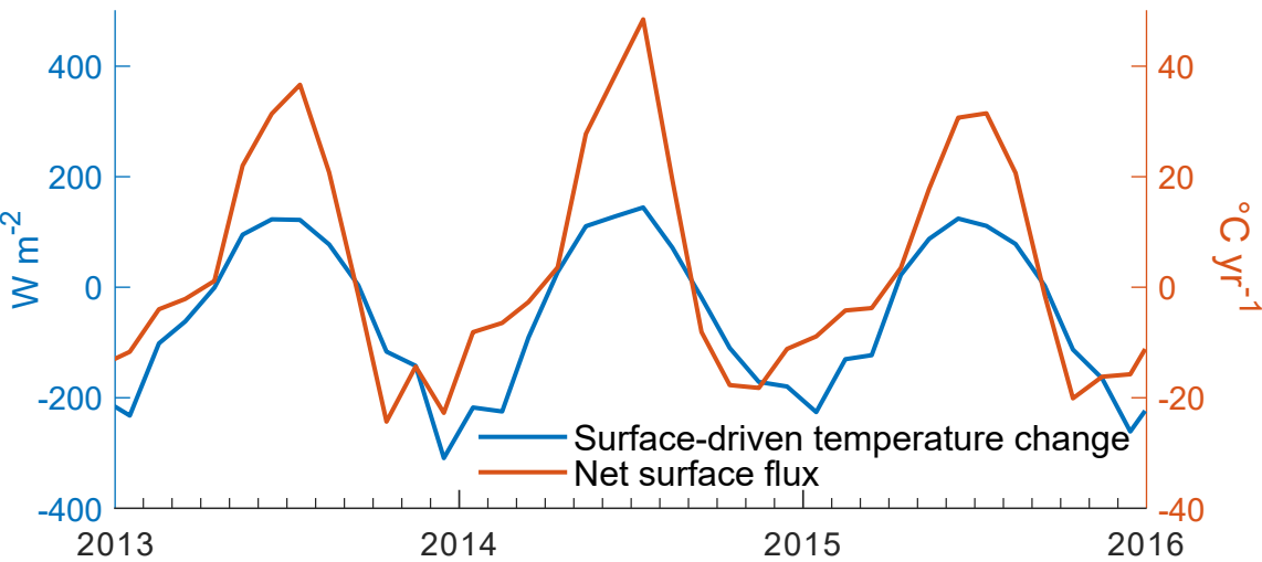
(a) Net surface heat flux
