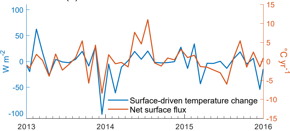
(a) Net surface heat flux anomalies
