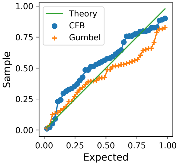
(c) PP plot, Observations
