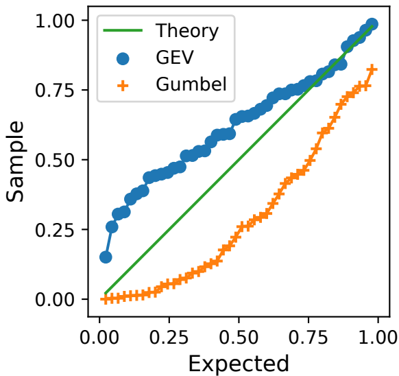
(a) PP plot, Simulation
