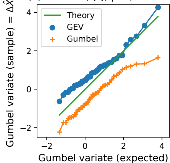
(b) VdBK08 (QQ) plot, Simulation
