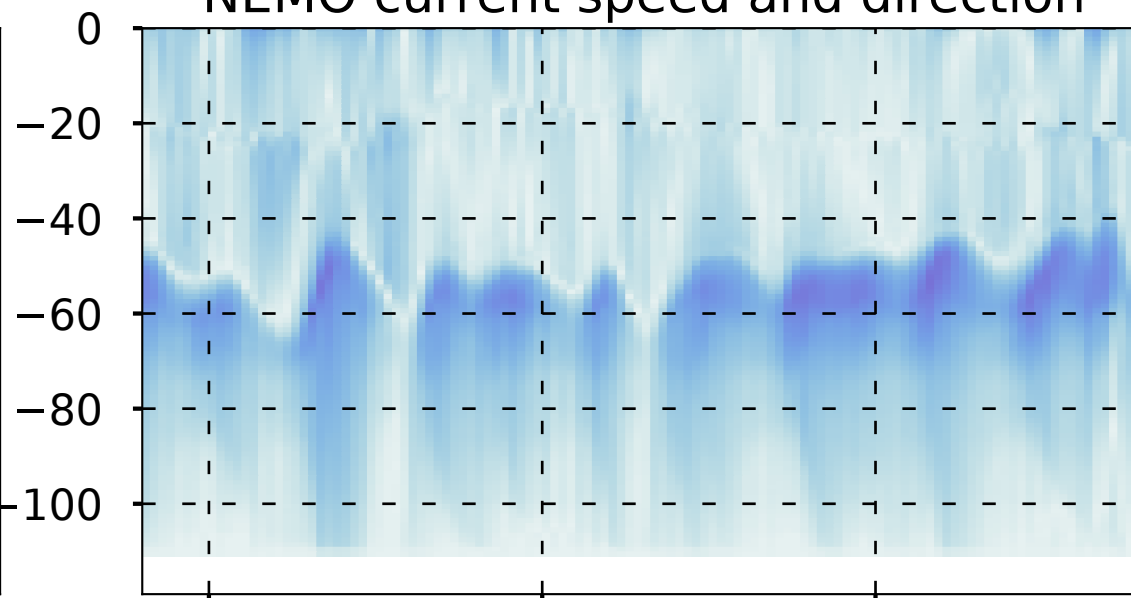
NEMO current speed and direction
