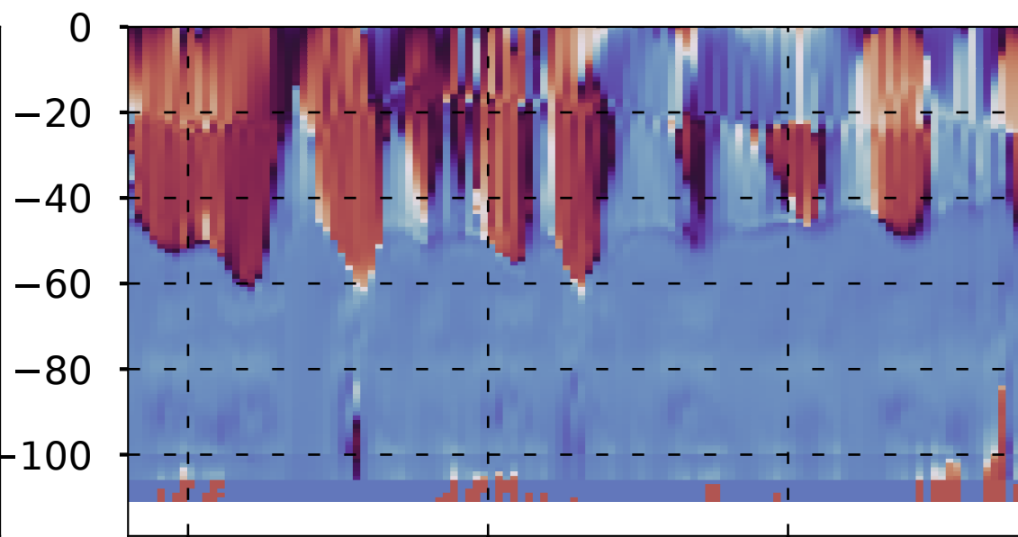
NEMO temperature and salinity
