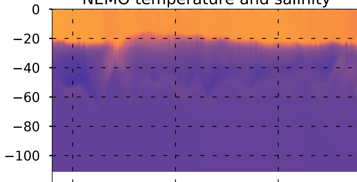
NEMO temperature and salinity
