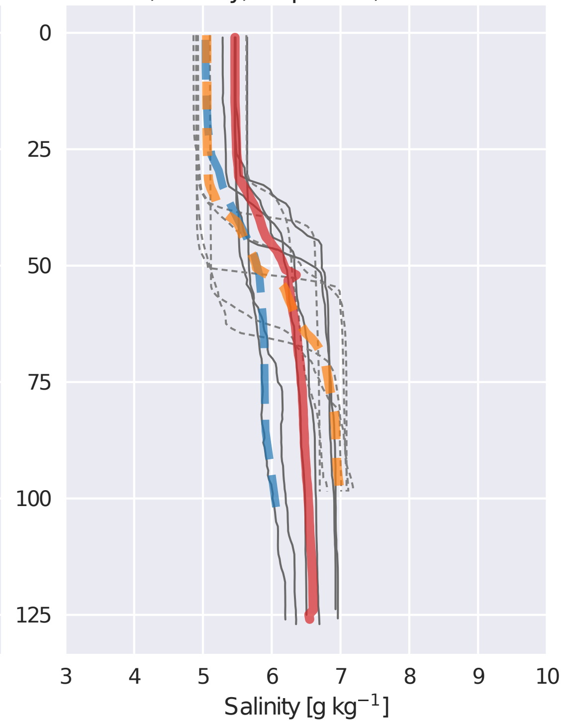
F64, salinity, 32 profiles, 2013-2017
