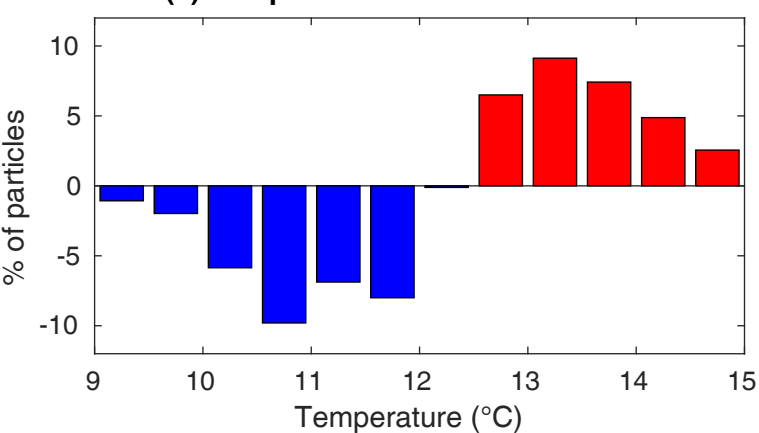
(e) Temperature difference 2010 - 1992
