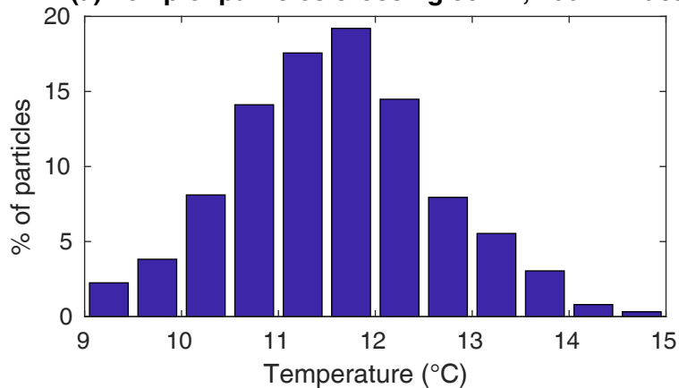
(c) Temp of particles crossing 30° W, 2010 hindcast
