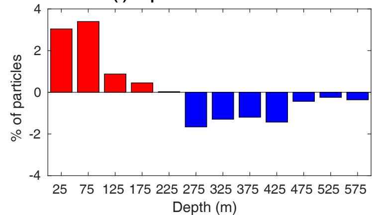
(f) Depth difference 2010 - 1992
