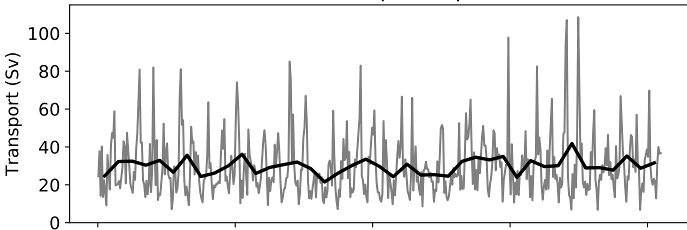
(b) Ekman transport
