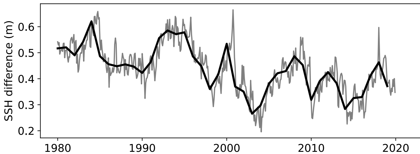
(c) SSH difference 45 - 60 ° N
