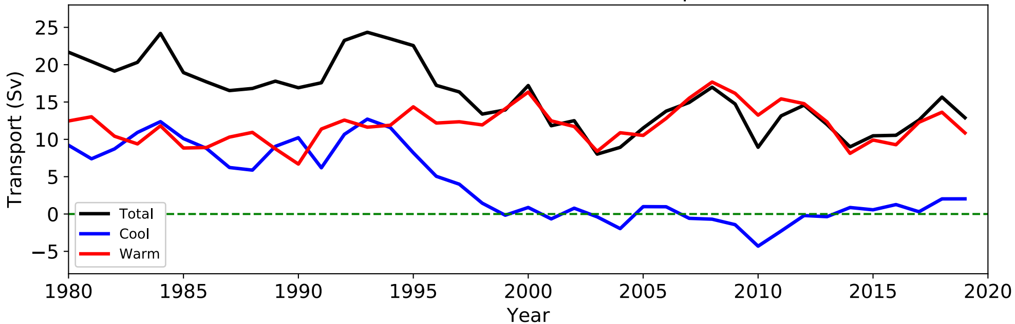
(b) Total eastward volume transport
