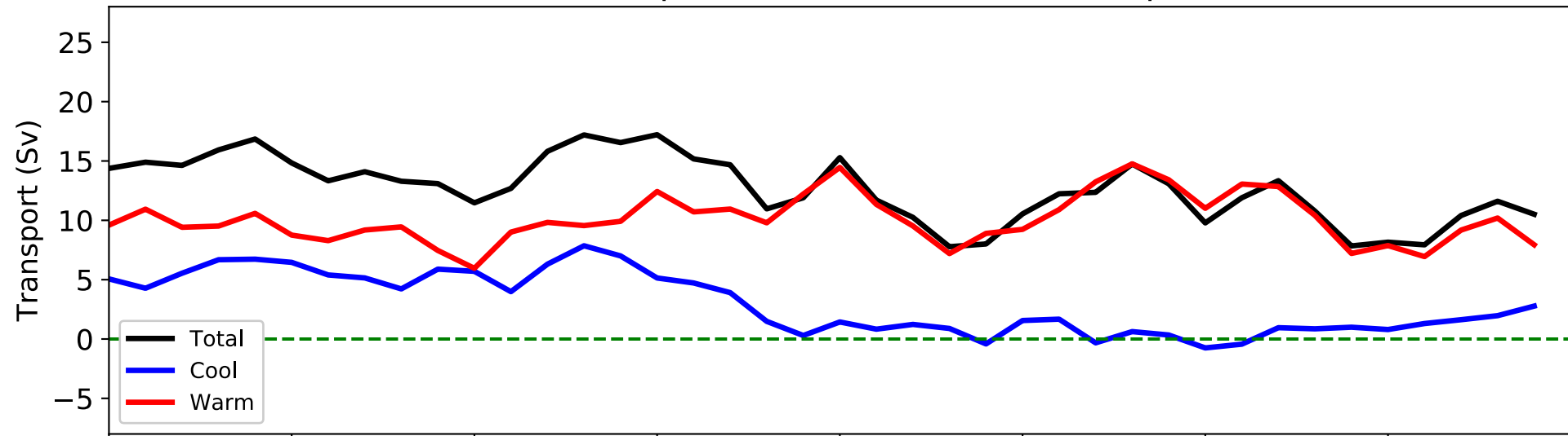
(b) Total eastward volume transport
