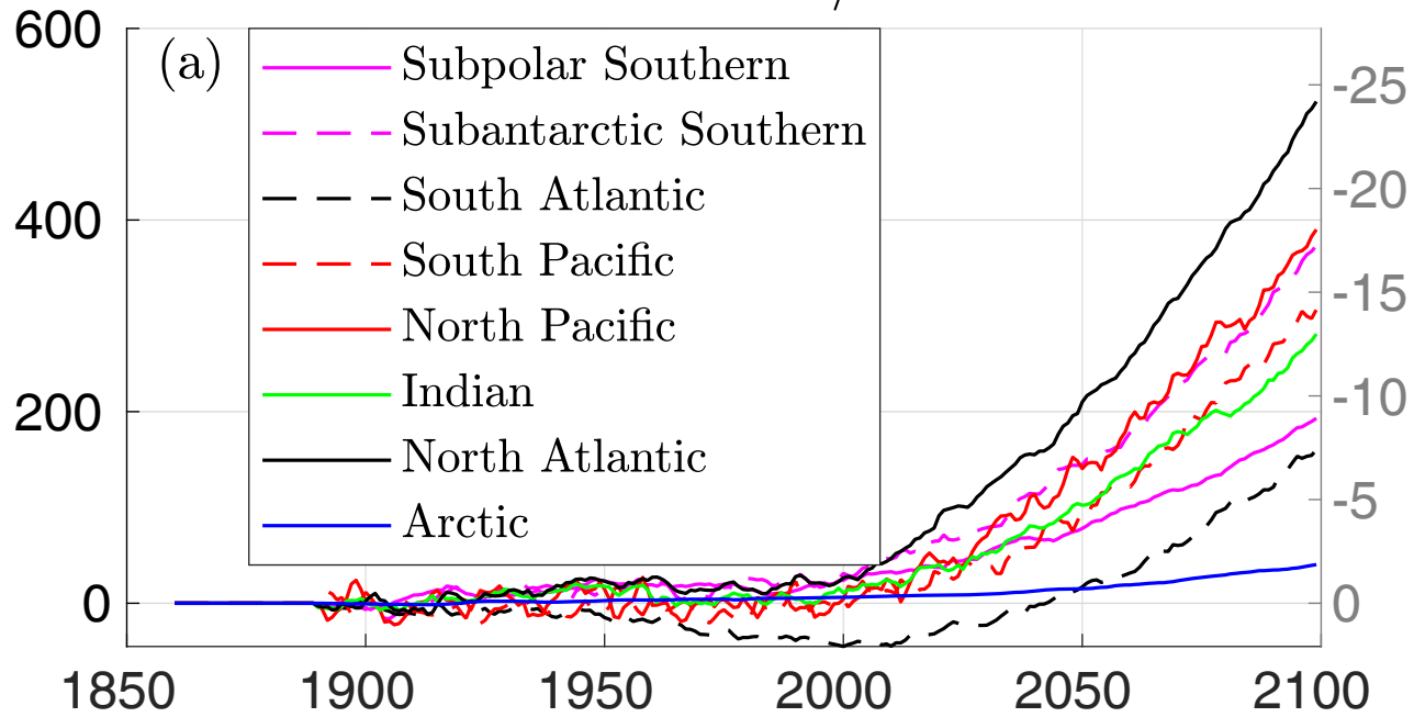
Excess Heat / ZJ
