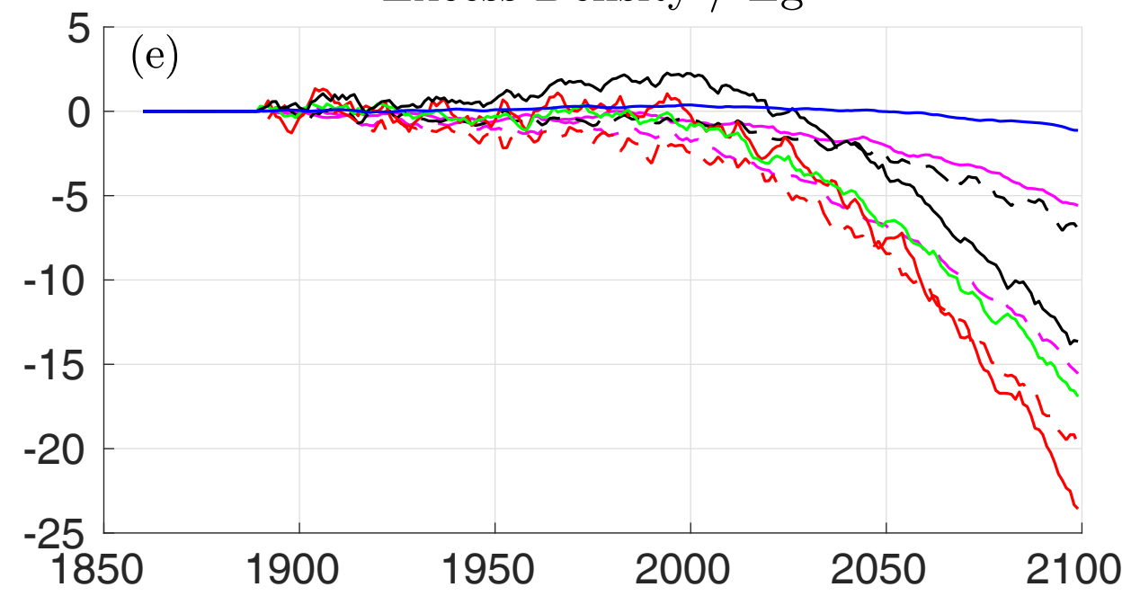
Excess Density / Eg
