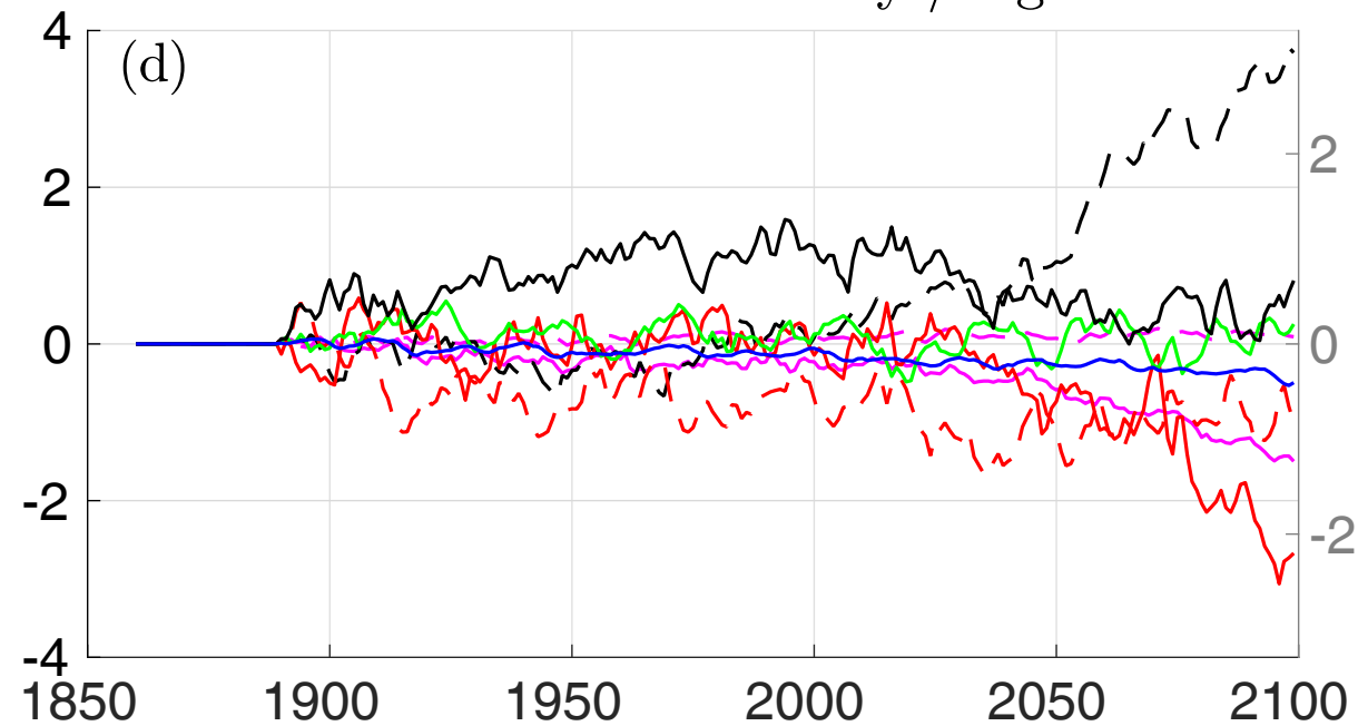
Redistributed Salinity / Eg
