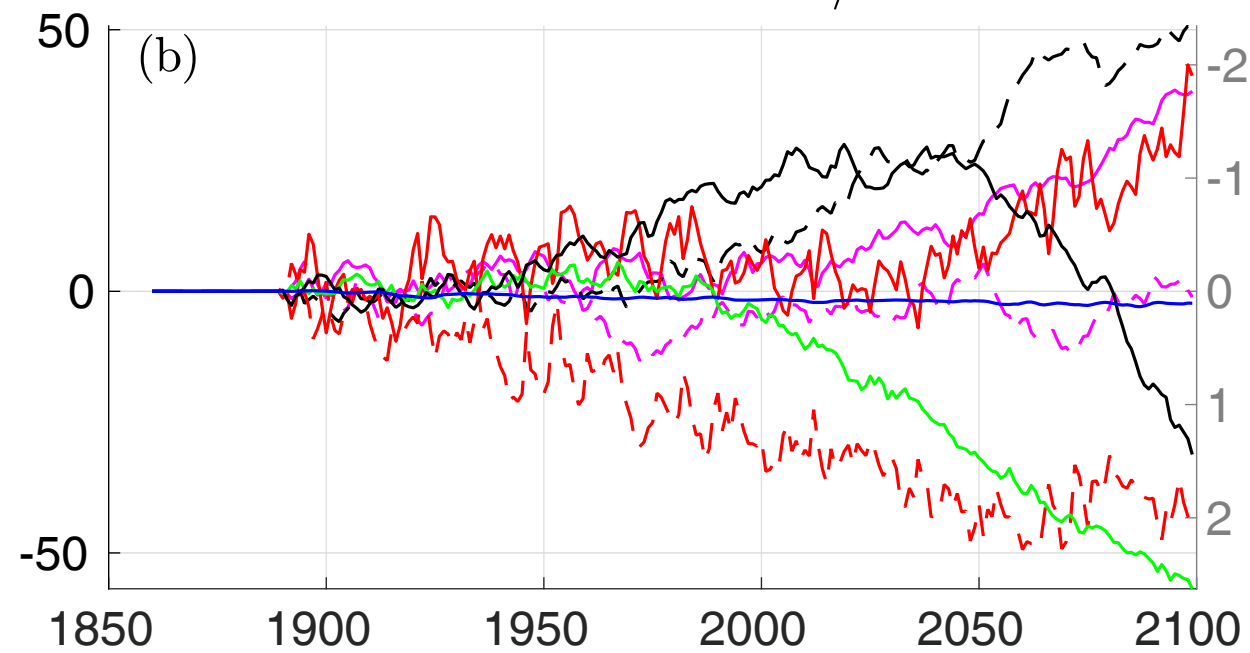
Redistributed Heat / ZJ
