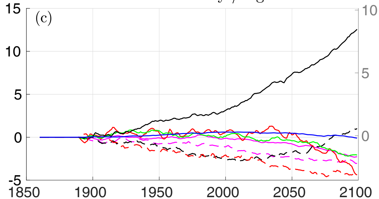
Excess Salinity / Eg
