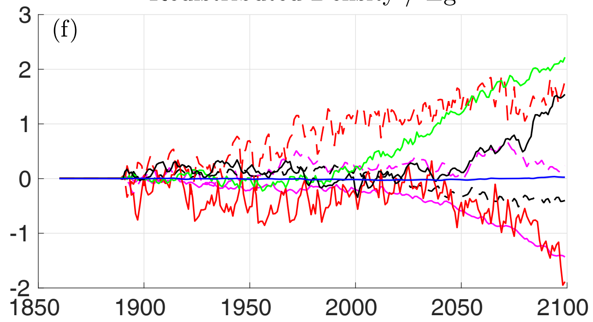
Redistributed Density / Eg
