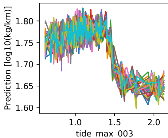
Importance ranking: 5
