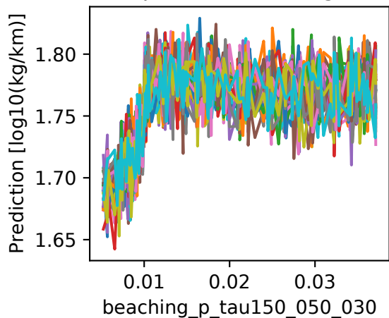
Importance ranking: 10
