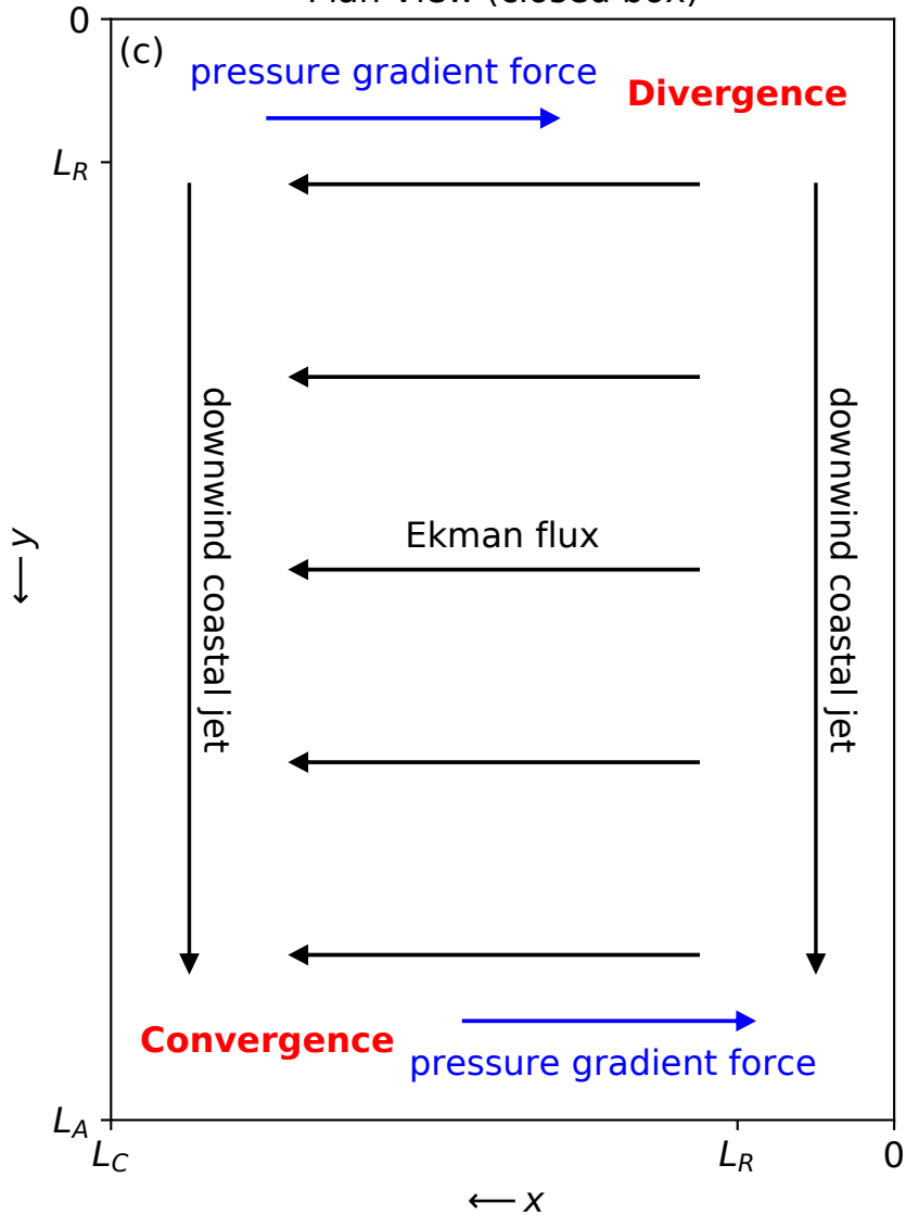
Plan View (closed box)
