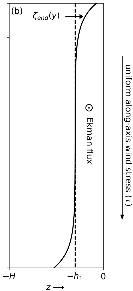
Along-axis section (infinite channel)
