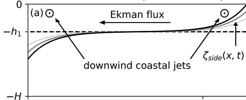
Cross-axis section (infinite channel)
