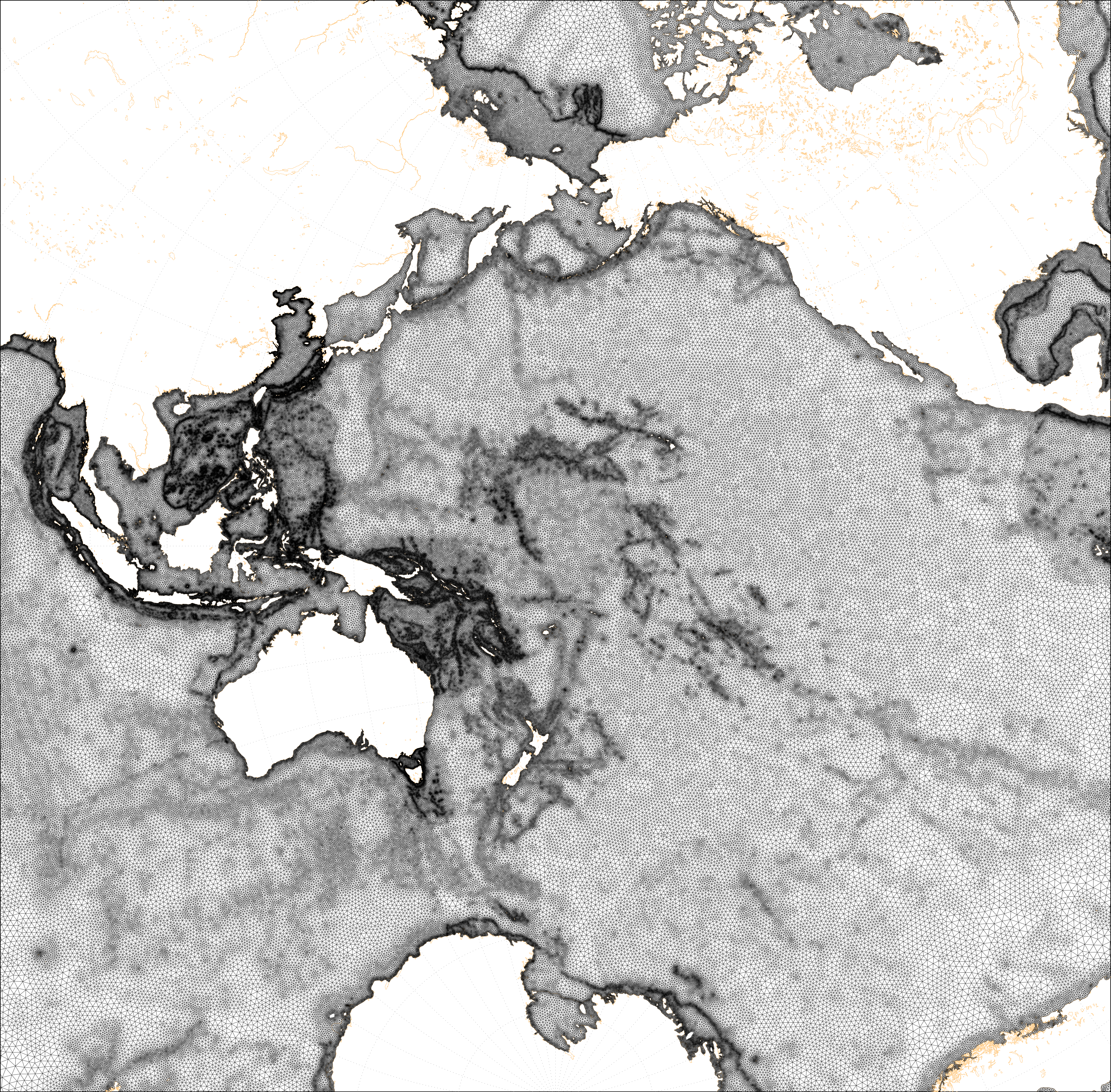
FES2014 finite element mesh with a stereographic projection centered on 0°N 180°E. Mesh details can be displayed by zooming in.
