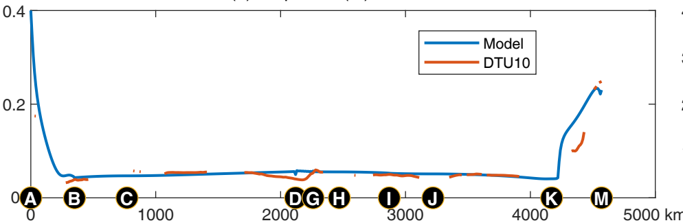
(a) Amplitude (m) of K_1 tide
