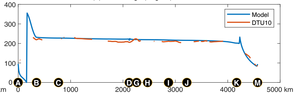
(b) Phase lags (degree) of K_1 tide
