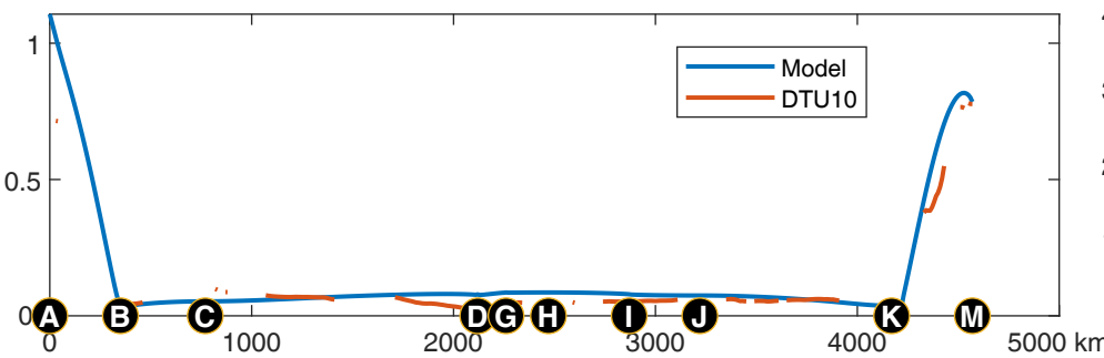
(c) Amplitude (m) of M_2 tide
