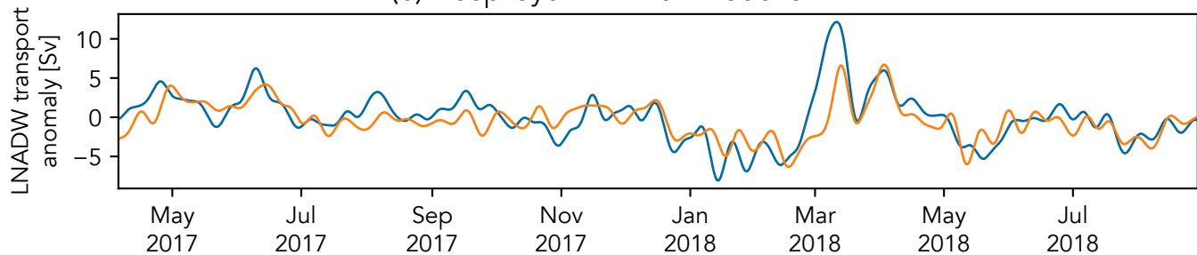
(b) Deep layer + Ekman model of LNADW
