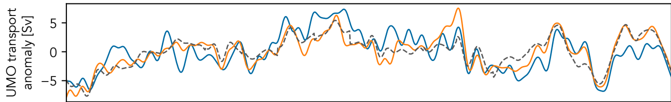
(a) Four-layer model of UMO
