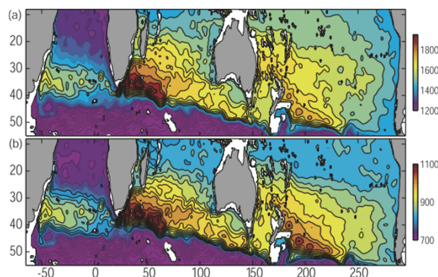
Figure 16. The interbasin supergyre system for the Pacific Ocean and Indian Ocean as shown by the depth-integrated steric heights (a) P_{0/2000} and (b) P_{400/2000} derived from the CARS climatological temperature and salinity fields. The contour interval in (a) is 50 \text{ m}^2 , and it is 25 \text{ m}^2 in (b). Taken from Ridgway and Dunn (2007).
