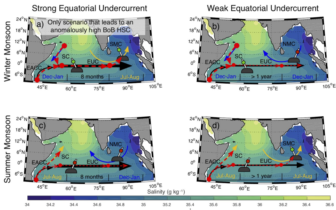
Figure 19. Seasonal circulation pathways in the northern Indian Ocean, or the railroad switch schematic, on subsurface (90 m) salinity climatology (psu; shaded) from the Argo optimally interpolated product for the four Equatorial Undercurrent scenarios: (a, b) winter monsoon and strong (weak) Equatorial Undercurrent and (c, d) summer monsoon and strong (weak) Equatorial Undercurrent. Dashed red arrows indicate high-salinity advection. BoB stands for Bay of Bengal, HSC stands for high-salinity core, SMC stands for Southwest Monsoon Current, SC stands for Somali Current, EUC stands for Equatorial Undercurrent, EACC stands for East African Coastal Current. Figure taken from Sanchez-Franks et al. (2019).
