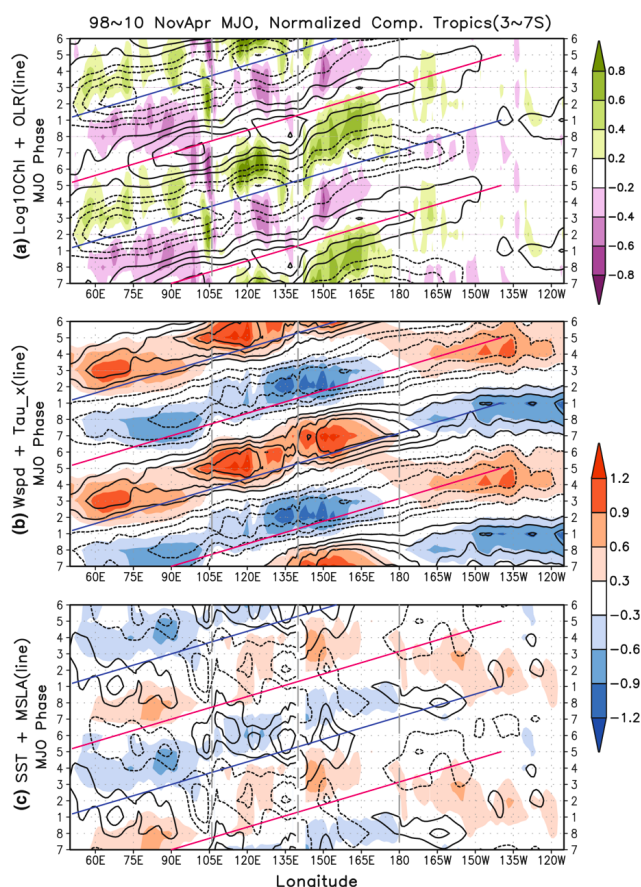
Figure 8. MJO composite evolution for the boreal winter (November–April) averaged over latitudes 3–7° S for the period of 1 November 1997 to 31 October 2010: (a) \text{Log}_{10}\text{Chl} from SeaWiFS satellite observations (shaded) and satellite-derived outgoing longwave radiation (contour); (b) wind speed (shaded) and zonal wind stress (contour), both from the cross-calibrated multiplatform (CCMP) data set; and (c) NOAA-OI satellite SST anomalies (shaded) and AVISO mean sea level anomaly (contour). All contour intervals match shading levels in (c) , and a solid (dashed) line indicates positive (negative) values. All variables are normalized, and the same MJO composite is repeated for two cycles for convenience. There are between 127 and 227 events in the composite for each MJO phase. Diagonal red lines indicate peak signals of positive OLR, and blue lines indicate negative OLR peak; these are guides for the MJO propagation. The relative location of each propagation line in all panels is the same. The left and centre dashed vertical grey lines indicate the western and eastern boundary of the Maritime Continent, respectively, and the right grey line is on the International Date Line where chlorophyll a propagation stops. From Jin et al. (2013a).
