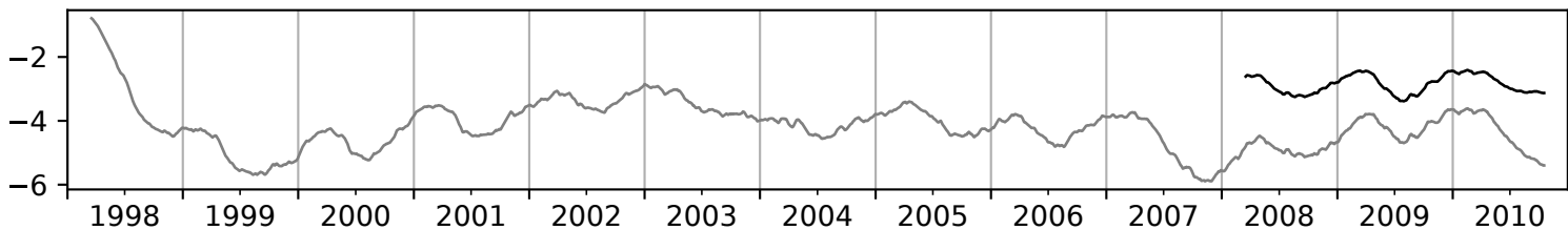
(g) Air-sea CO 2 flux (anomaly from free run)
