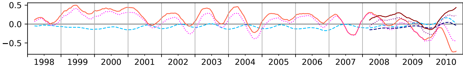
(g) Air-sea CO 2 flux (anomaly from free run)
