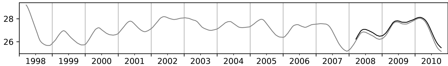
(c) SST (anomaly from free run)
