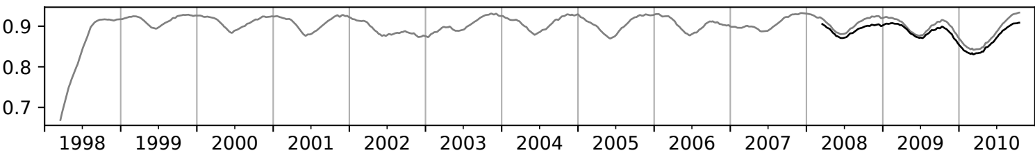
(e) Primary production (anomaly from free run)
