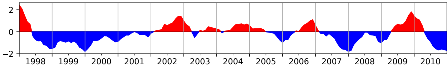
(b) SST (free run)
