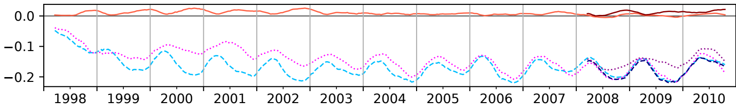
(f) Air-sea CO 2 flux (free run)
