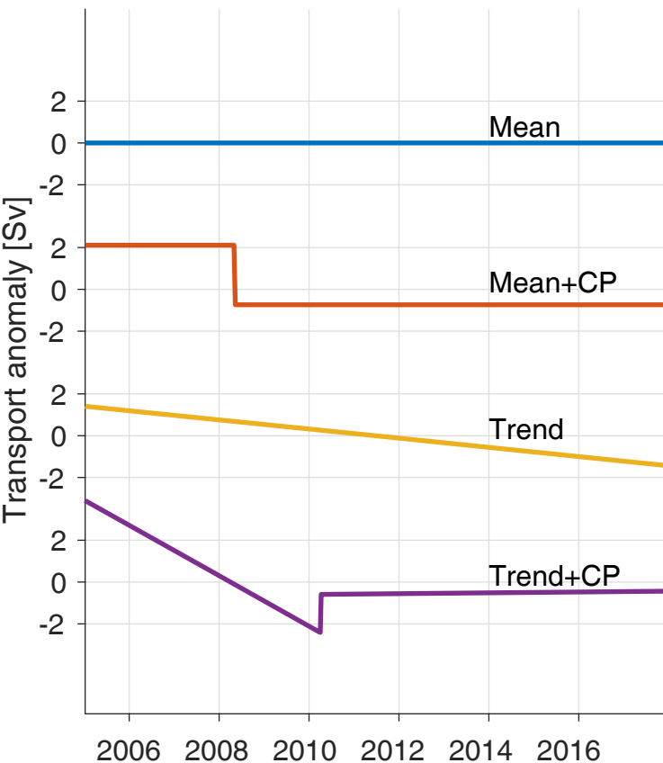
(a) Change point and mean or trend
