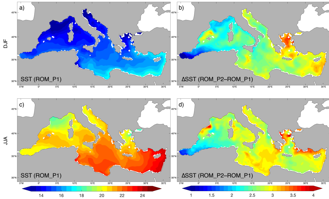
Supplementary figure: Mean SST (in °C) in winter (DJF, top left) and summer (JJA, bottom left) averaged over the 1976-2005 period. Difference between mean SST (in °C) RCP8.5 projection (2070-2099, ROM_P2) and present climate (1976-2005, ROM_P1) for DJF (top right) and JJA (bottom right).
