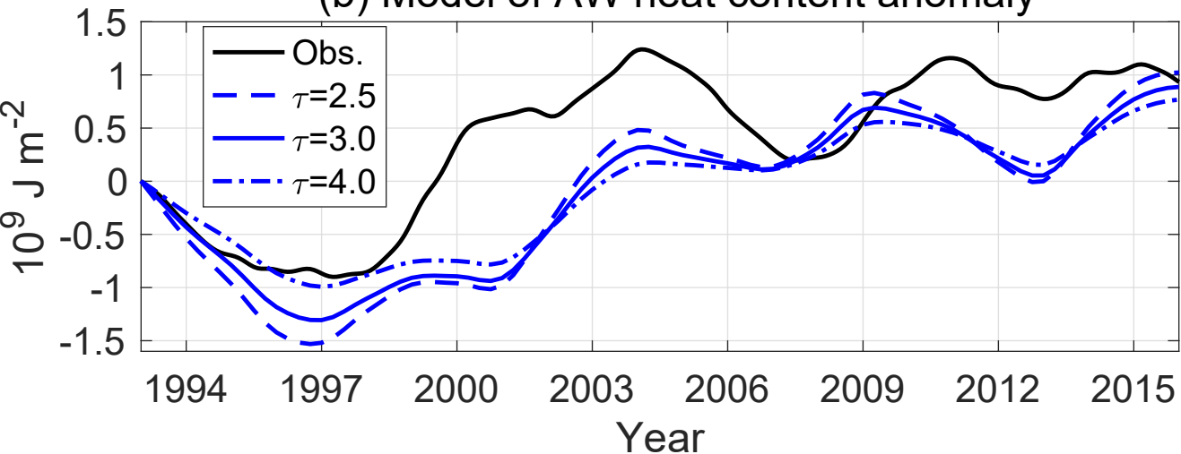
(b) Model of AW heat content anomaly
