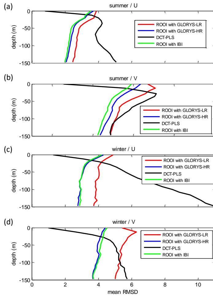
Figure S11. Mean RMSDs related to all the data-reconstruction methods for each depth considering the entire grid. For the summer period (a, b) and for the winter period (c, d). U in a, c and V in b, d.
