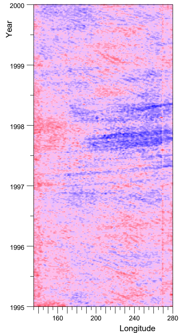
Model - observations
