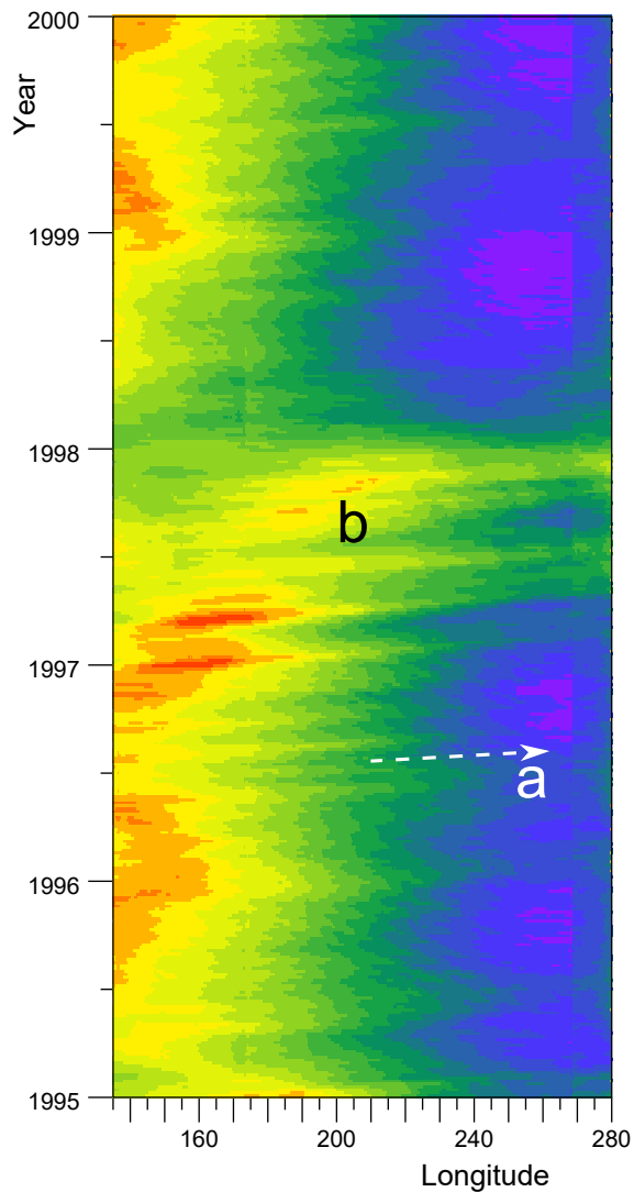
Model
