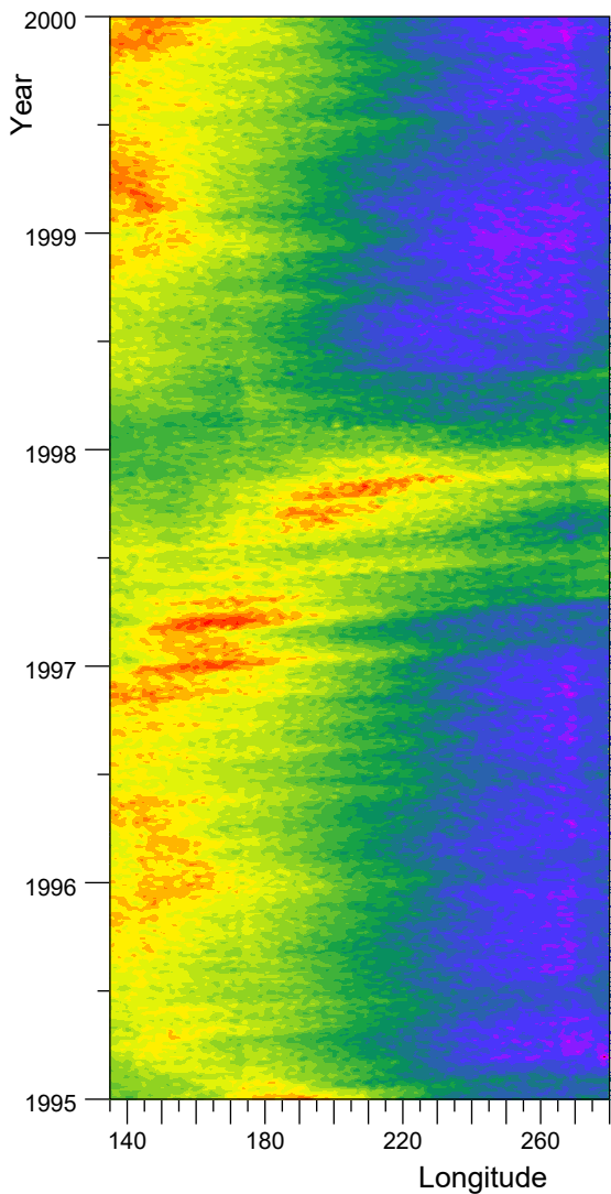
Observations
