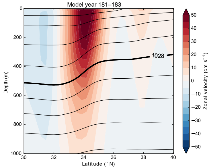
(b) Model year 181–183
