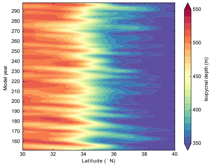
(c) Isopycnal depth, 1028 \text{ kg m}^{-3}
