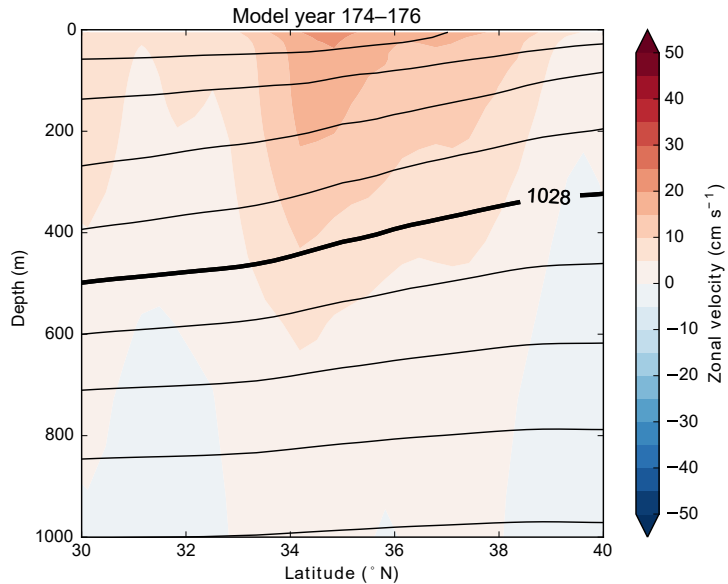
(a) Model year 174–176
