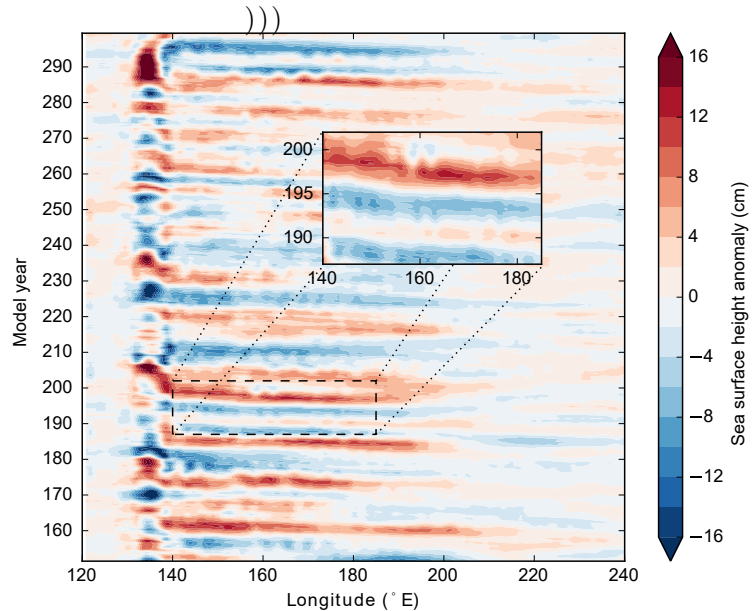
(a) SSH Hovmöller
