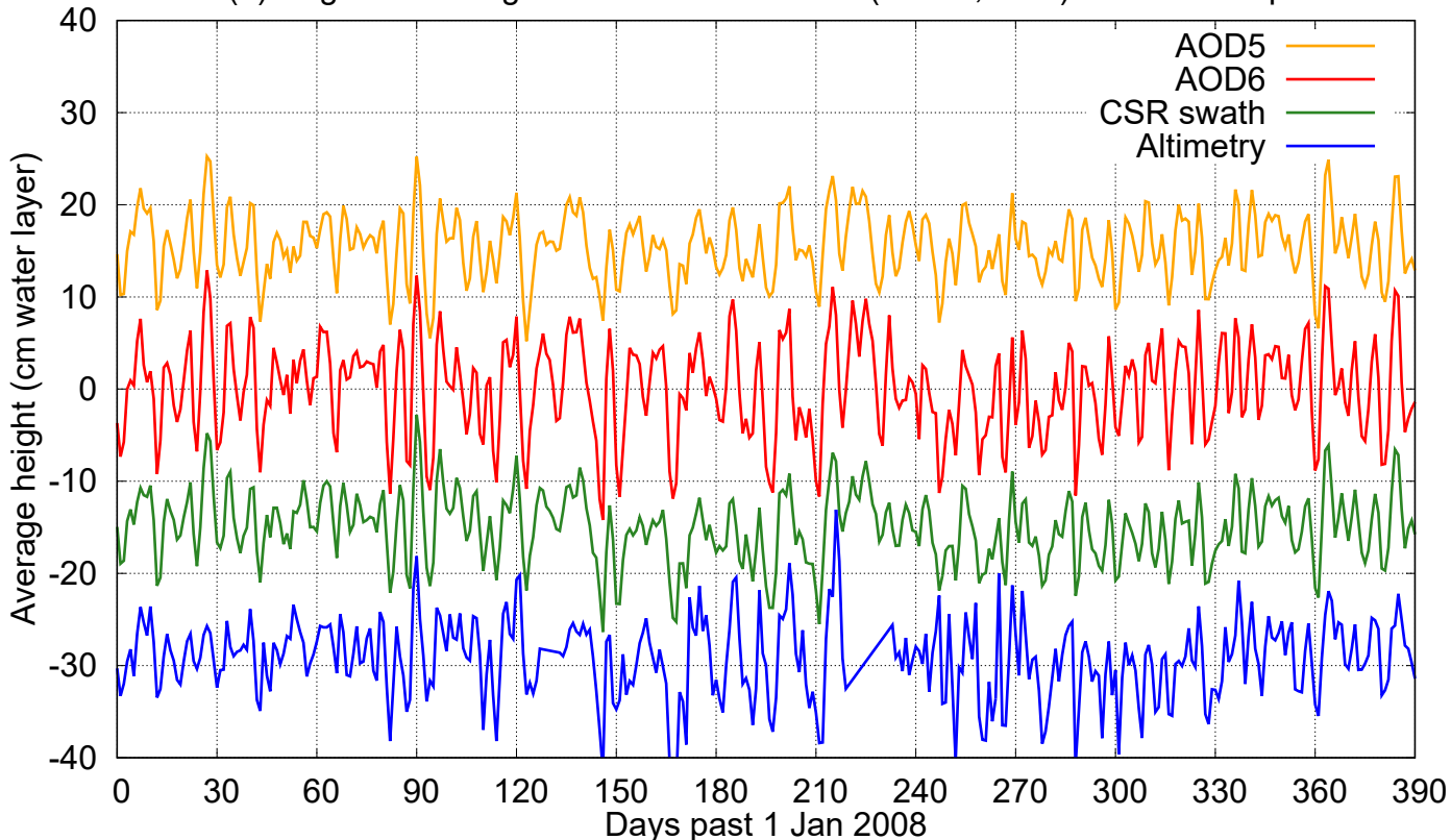
(b) Regional averaged time series over the (210° E, 60° S) anomalous spot
