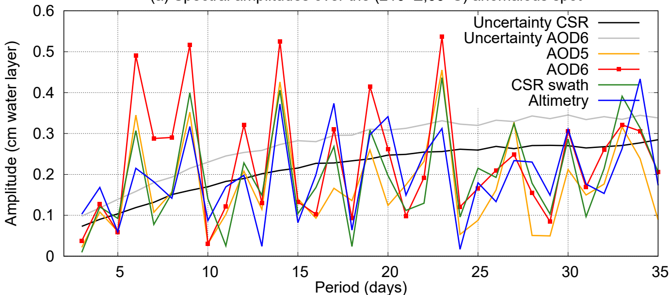
(a) Spectral amplitudes over the (210° E, 60° S) anomalous spot
