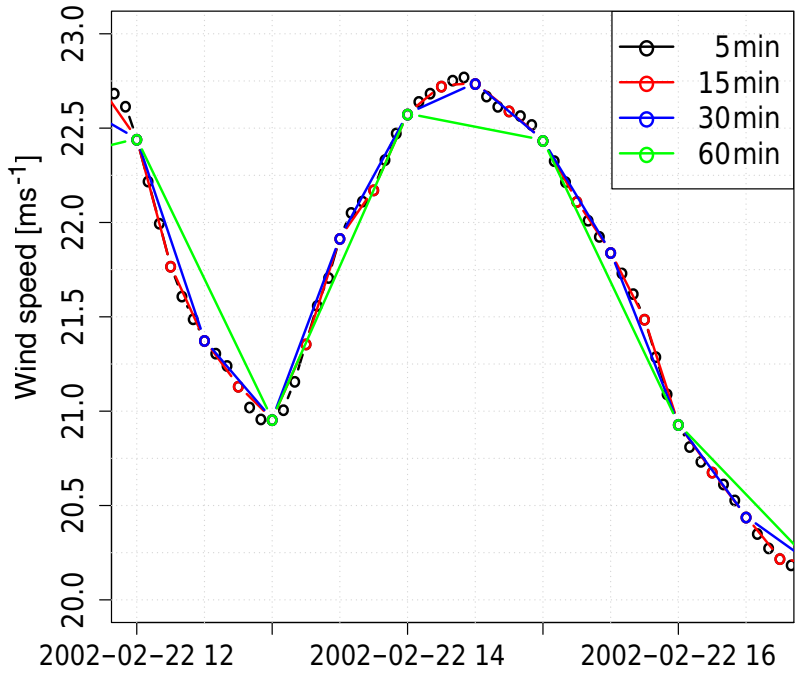
(a) WRF 0.063°
