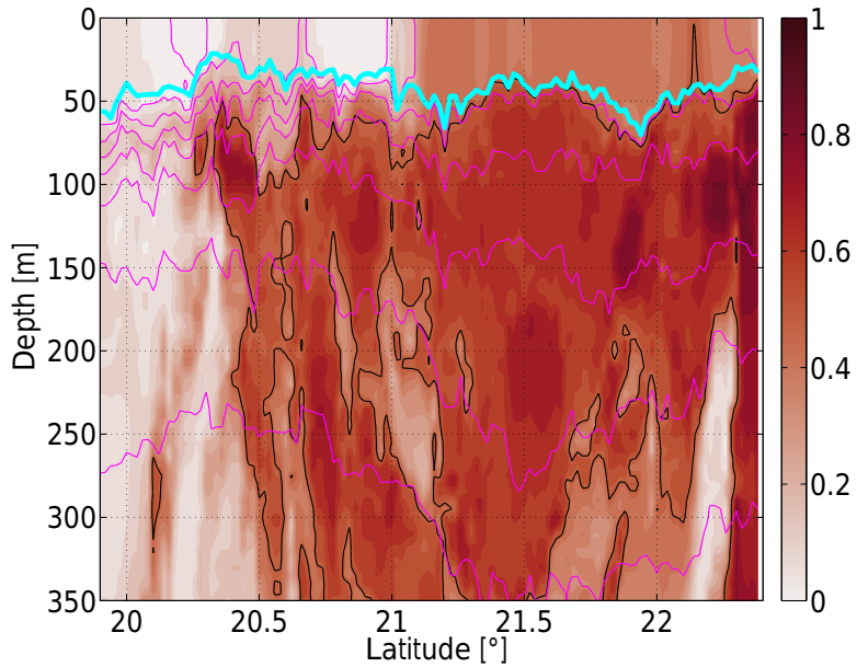
(b) Fraction of NACW [ ^{\circ} ] with 0.5 contour in black
