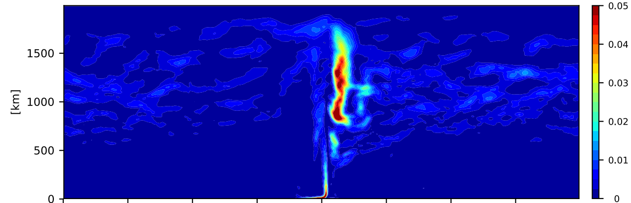
(e) EKE_{(0-500m)} [m^2s^{-2}] - R+R
