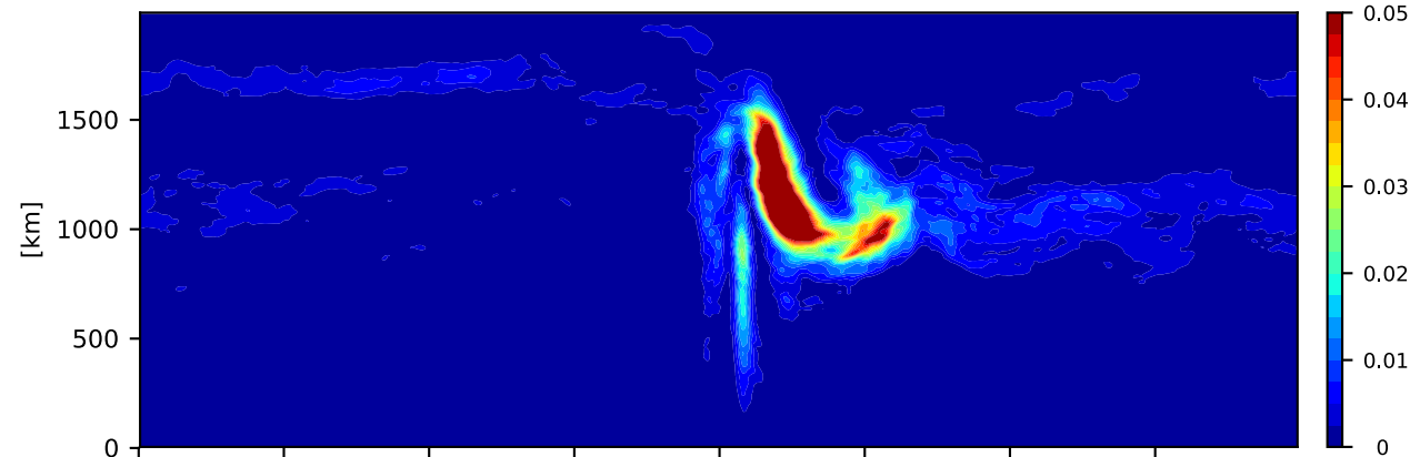
(b) EKE_{(0-500m)} [m^2s^{-2}] - R+F
