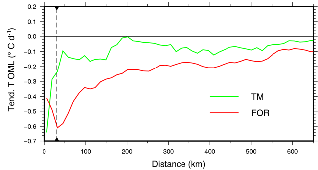
Figure 9. Mean values of the turbulent mixing (green) and surface forcing (red) tendency terms for temperature evolution in the OML at 10:00 UTC on 7 November. The values are radially averaged every 12 km from the medicane centre. The vertical dashed line indicates the radius of maximum wind.
