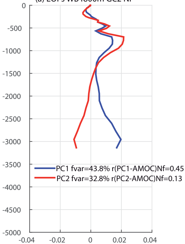
(a) EOFs WB f800m GC2 Nf
