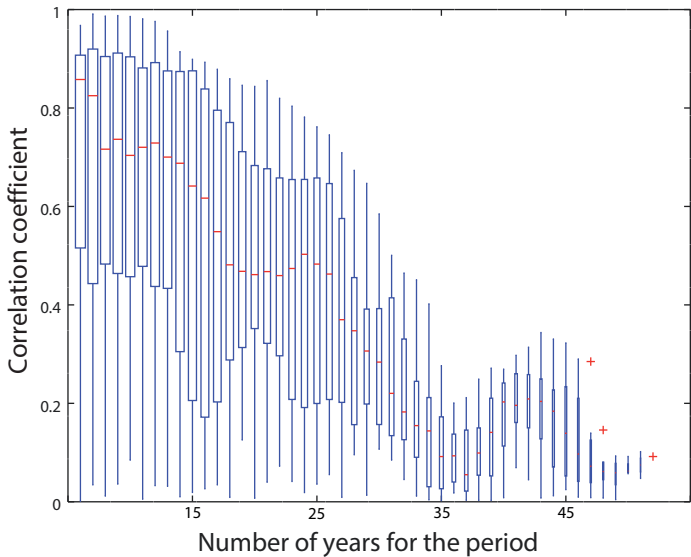
(a) r(\text{PC1-WB CTRL}, \text{PC1-WB WIND})
