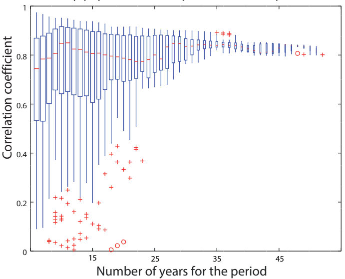
(b) r(\text{PC1-WB CTRL}, \text{PC1-WB BUOY})
