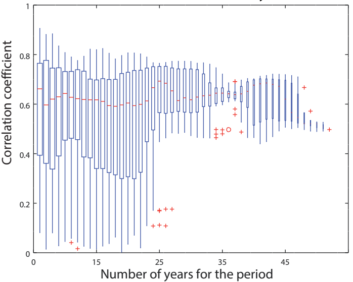
(c) r(\text{PC1-WB CTRL}, \text{AMOC}) > 2 \text{ yr}
