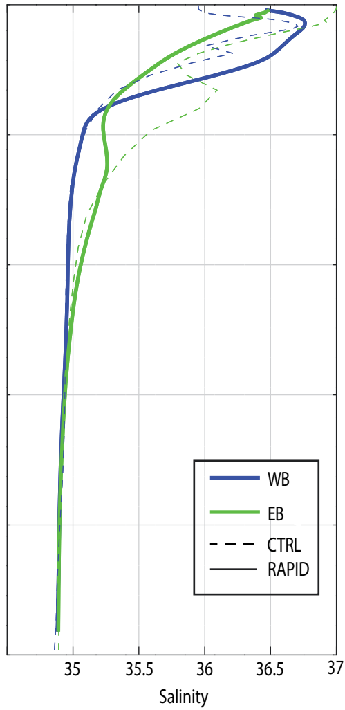
(b) Salinity 26° N
