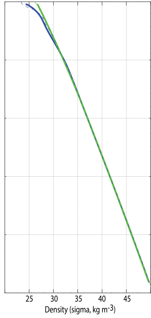
(c) Density 26° N
