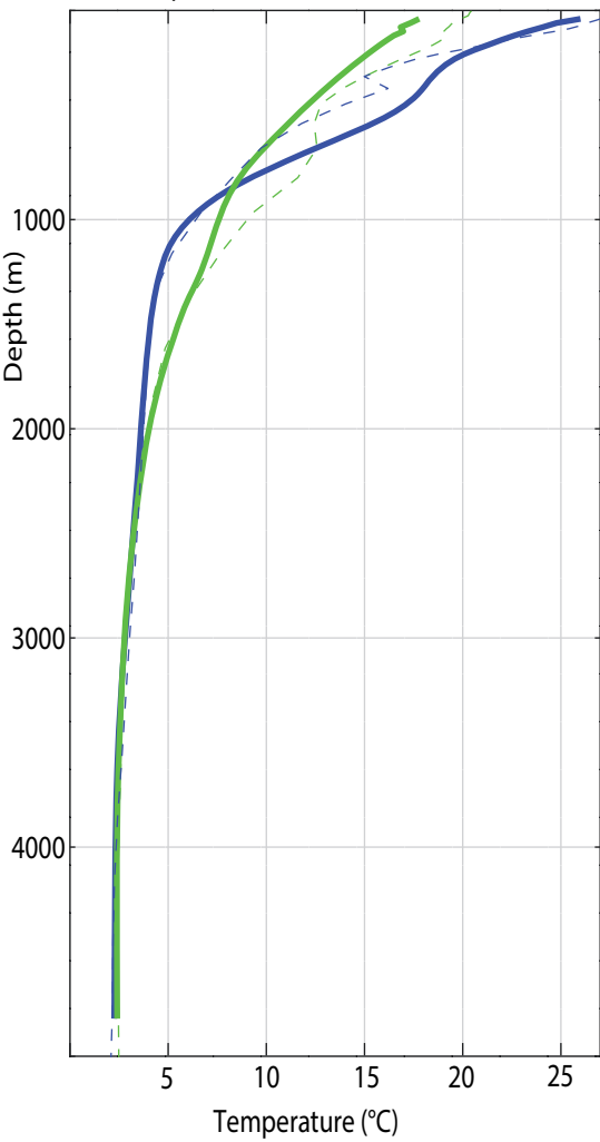
(a) Temperature 26° N
