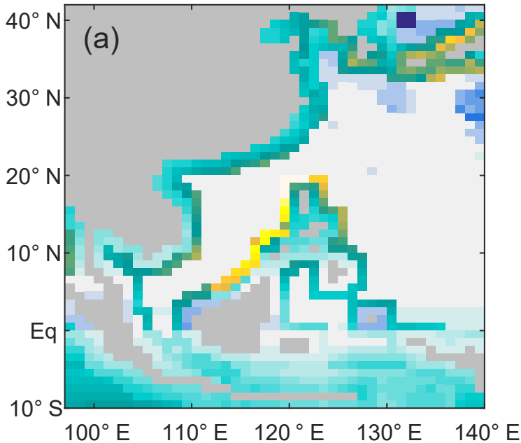
Ziska (2013) climatology
