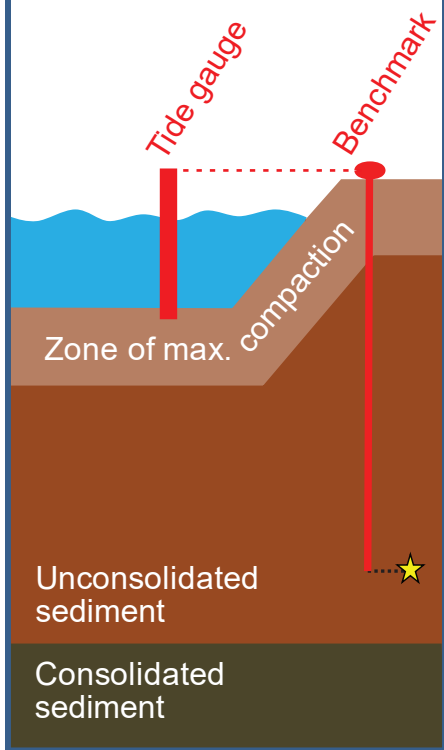
(c) Thick LECZ
