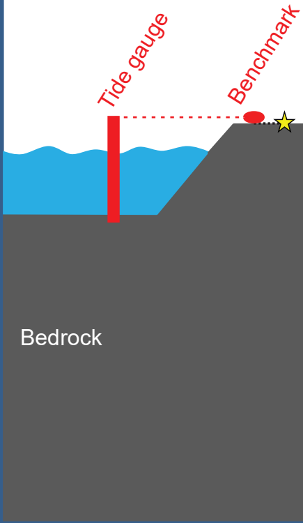
(a) Rocky coastline
