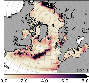
(a) Prior ensemble
