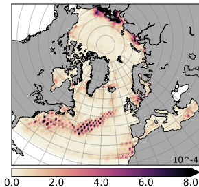
(c) Updated ensemble spectral + spatial localisation
