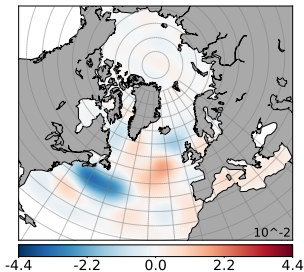
(c) Analysis increment : spectral + spatial localisation
