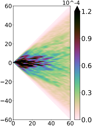
(a) Standard deviation
