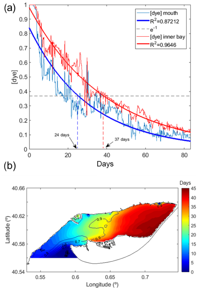
Figure 4. (a) Time evolution of the dye concentration at two points – at the bay mouth and inside the bay – and the corresponding exponential fitting (with the squared correlation shown in the legend) used to obtain the LFT for the C case. (b) The local e -flushing time for the C case (colour). The black contour shows the squared correlation obtained at each of the grid points.
