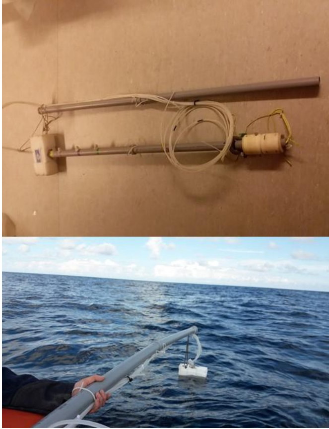
Supplementary Figure S3: Image of the High-volume Sampler for the Vertical (HSV) used to collect discrete samples for vertical profiles.
