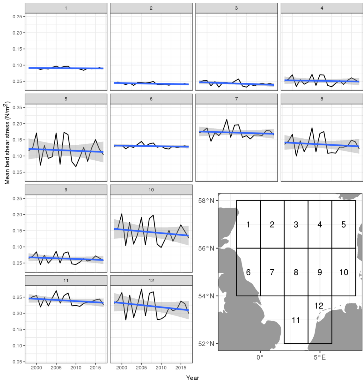
Figure S2: Trends in mean annual bed shear stress in the North Sea.
