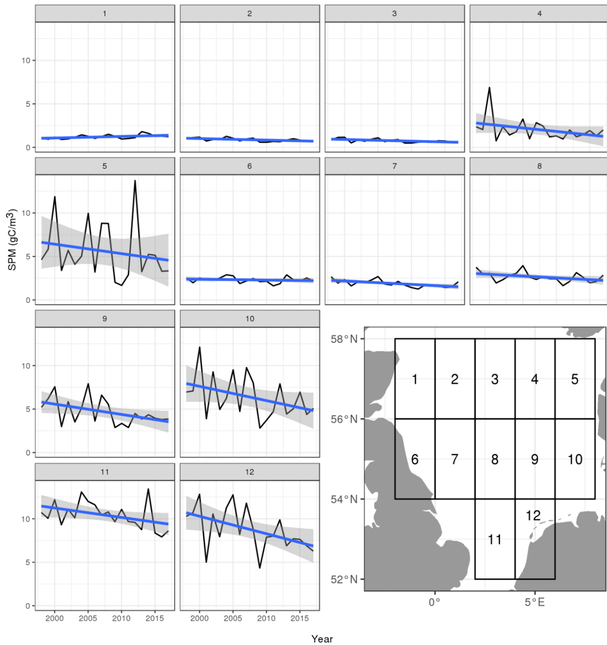
Figure S1: Trends in mean annual SPM in the North Sea (1997-2017) derived from remote sensing data.
