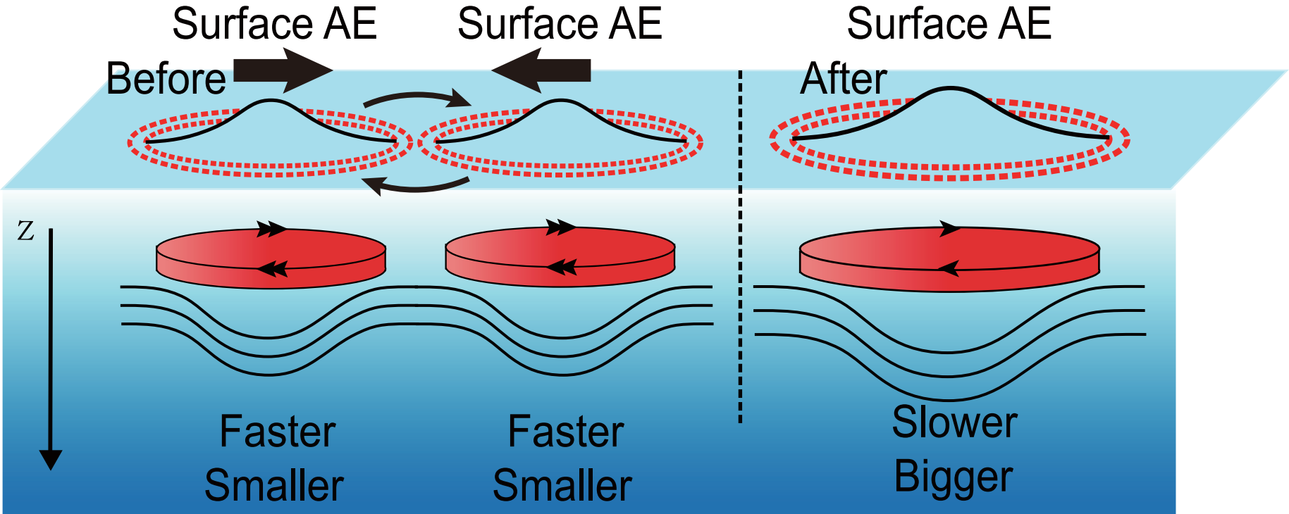
(a) Surface eddy merging event
