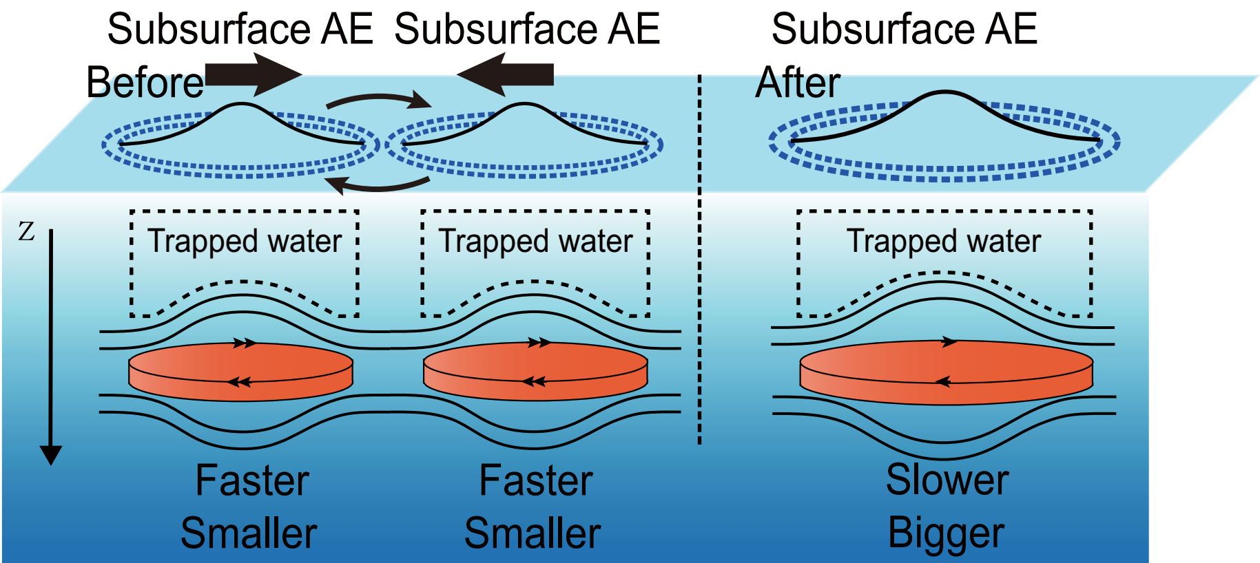
(b) Subsurface eddy merging event
