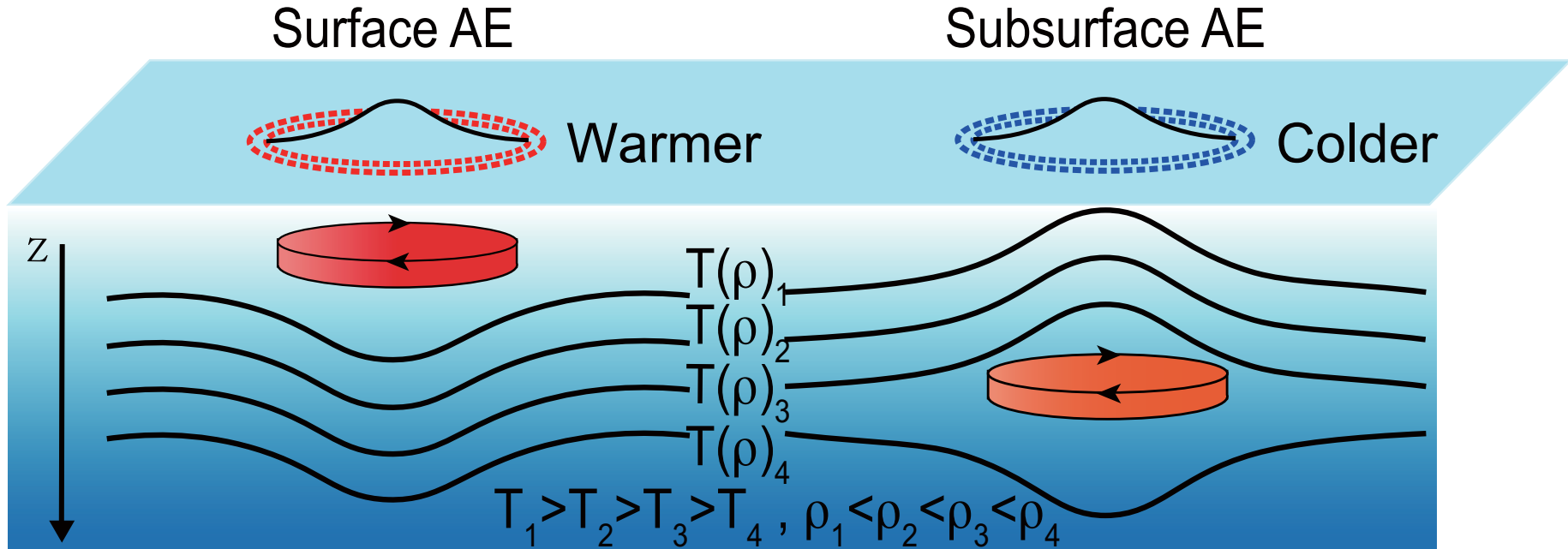
(a) Surface and subsurface AEs
